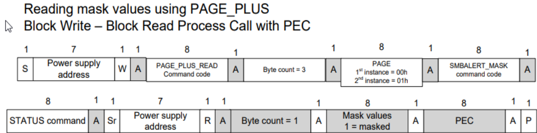
Figure 5. PAGE_PLUS_READ command.
