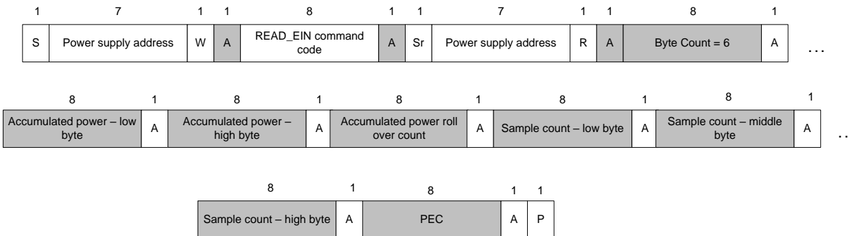
Figure 8. READ_EIN Command
